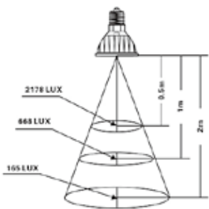
Cone to 50% of centre illuminance
