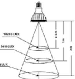
Cone to 50% of centre illuminance
